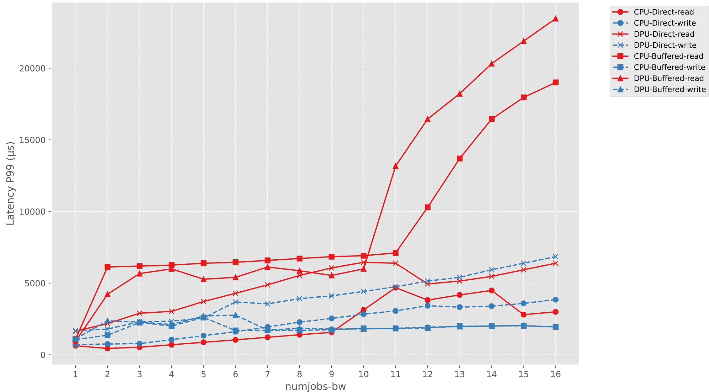
Latency P99 vs numjobs-bw (CPU vs DPU, Direct vs Buffered)
